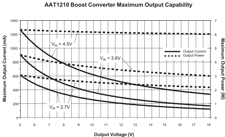
Figure 1: Maximum Output Power Vs. Output Voltage for T_{C(RISE)} = +50^\circ\text{C} (assumes TDFN34-16 paddle heatsinking; see Figures 6, 7, and 8).
