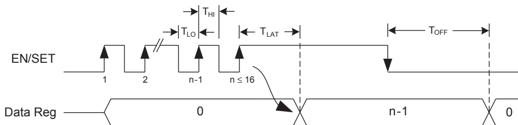
Figure 5: S 2 Cwire Timing Diagram.
