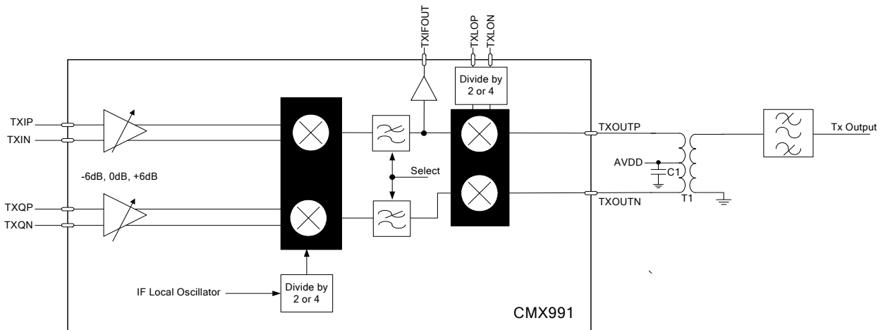
Figure 16 CMX991 Transmitter Architecture
