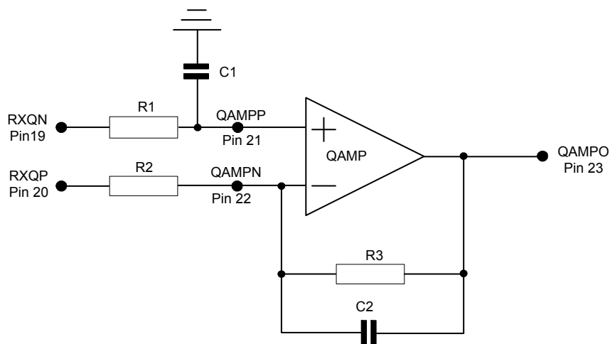
Figure 8 Example External Components – Receive I/Q Output
