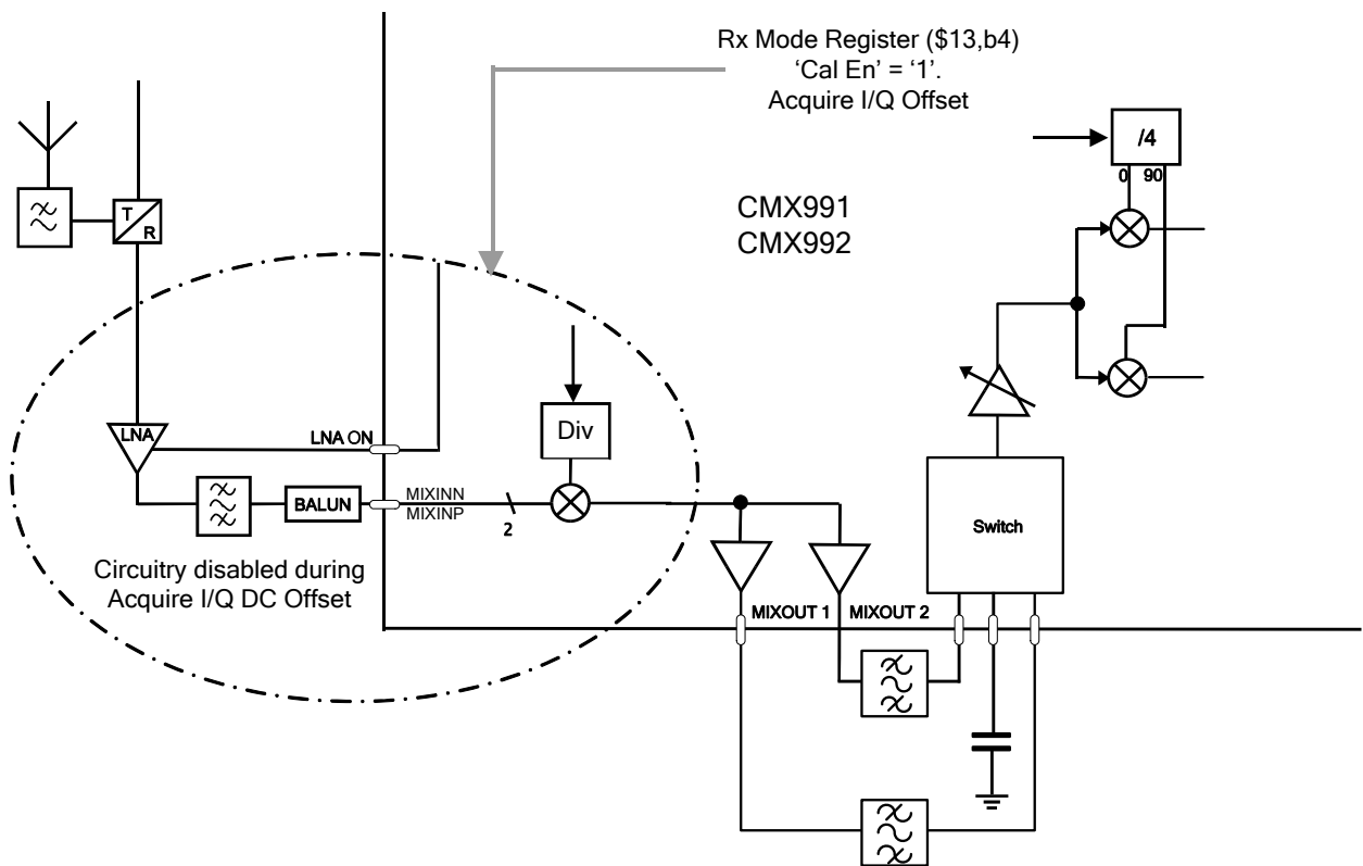
Figure 15 DC Offset Calibration Mode
