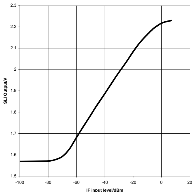
Figure 19 Typical SLI Performance (with the signal applied to IFIP1 or IFIP2 and terminated with a 50 ohm resistor)
