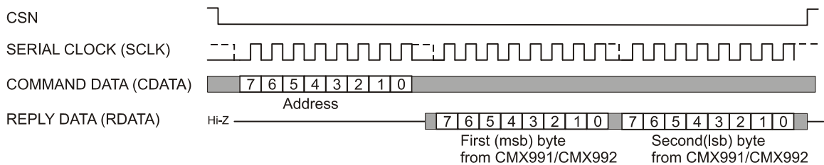
Figure 18 C-BUS Transactions
