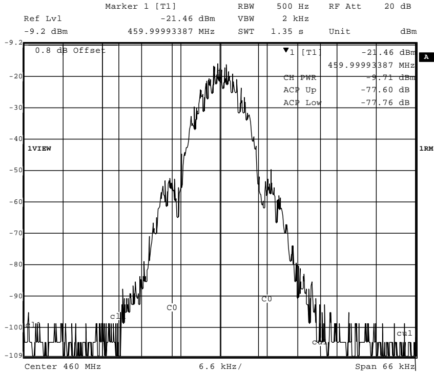
Figure 22 Tx Output with 9.6kbps GMSK from an EV9100 (TxIF = 90MHz, ACP ~ 77dBc)
