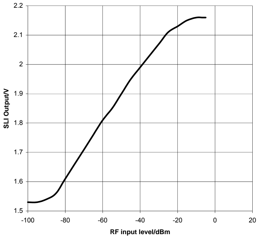
Figure 20 Typical SLI Performance in an Application Circuit (EV9920B) (Input 460MHz, 25kHz IF crystal filter: 45G15B1)
