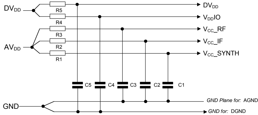
Figure 5 Recommended Power Supply Connections and Decoupling
