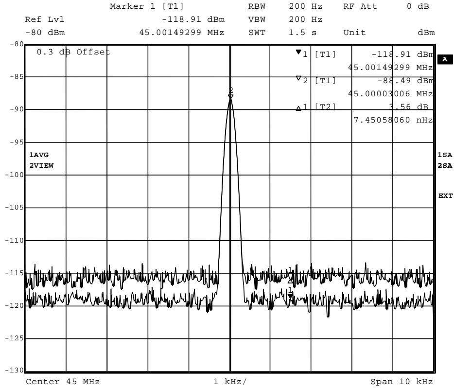
Figure 21 IF Output Response with and without blocking signal present
