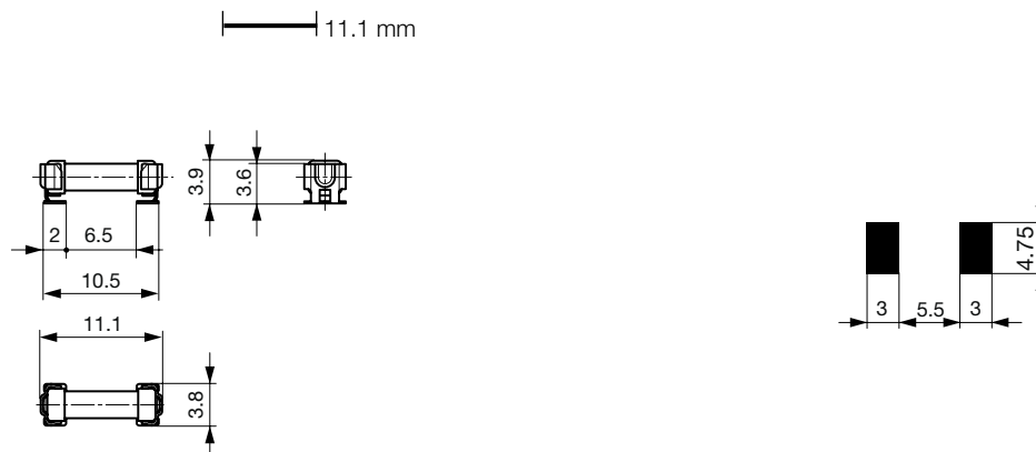
Soldering pads
