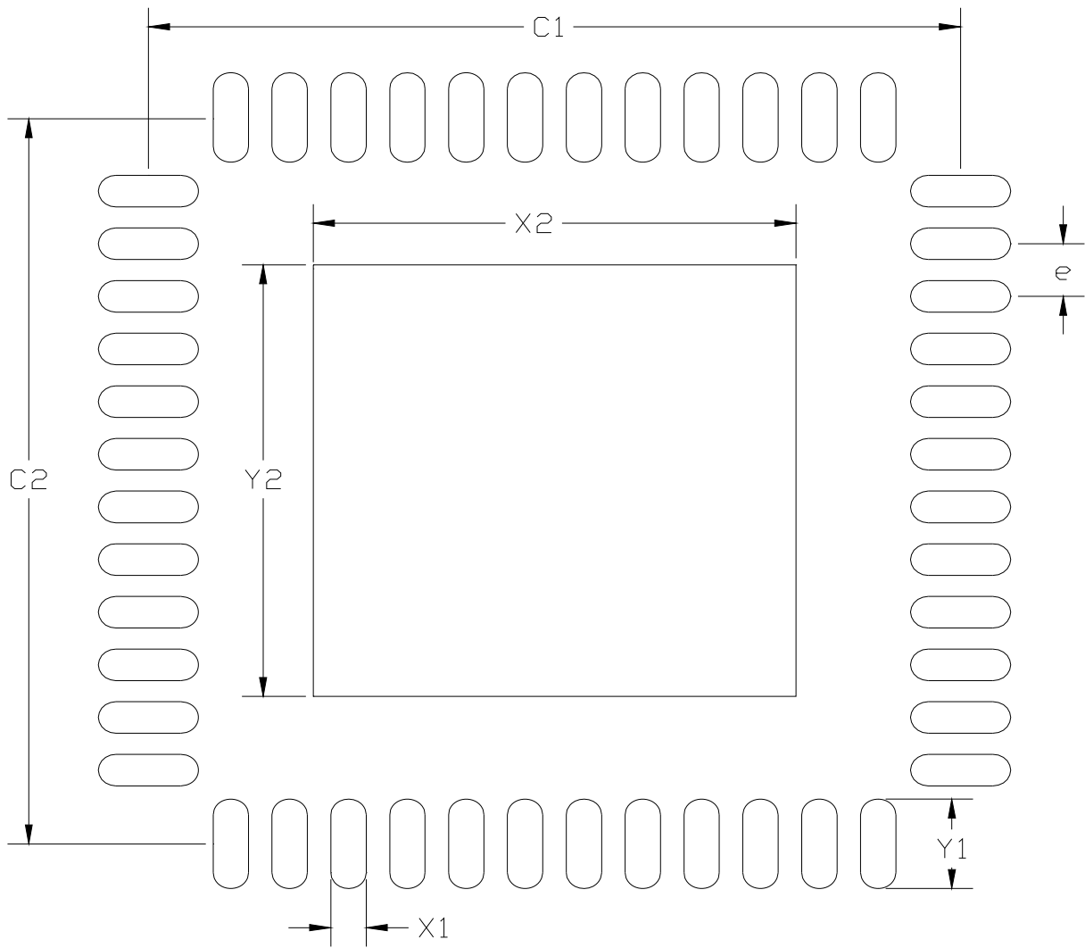
Figure 4.8. QFN-48 Landing Diagram
