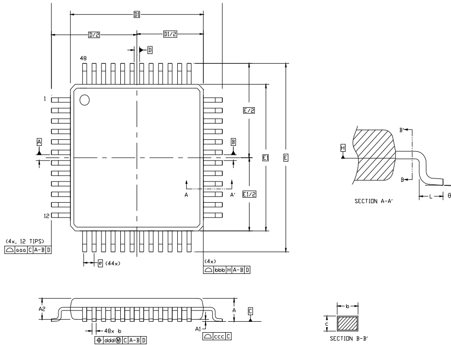
Figure 4.9. TQFP-48 Package Diagram
