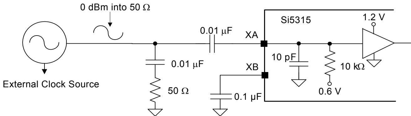
Figure 19. Sinewave External Reference Clock Input Example
