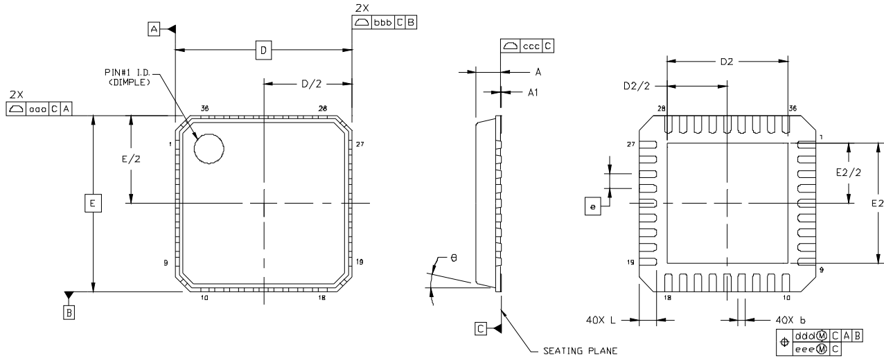
Figure 23. 36-Pin Quad Flat No-Lead (QFN)
