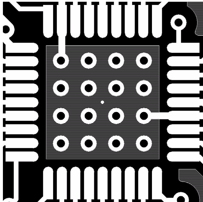
Figure 8. Ground Pad Recommended Layout
