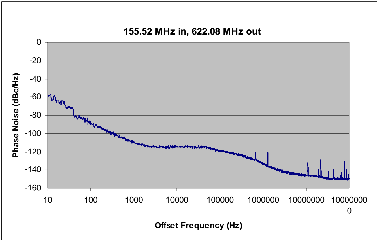
Figure 2. OTN/SONET/SDH Phase Noise
