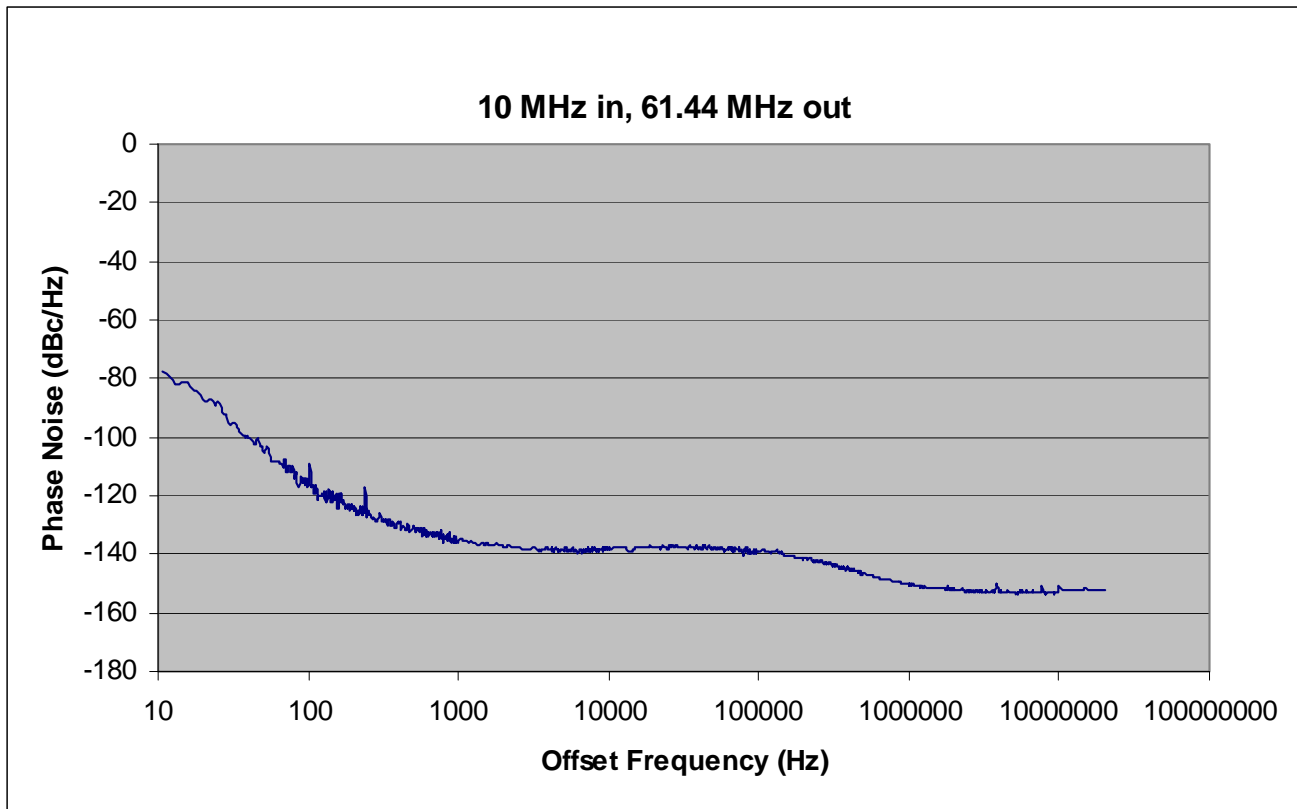
Figure 3. Wireless Base Station Phase Noise
