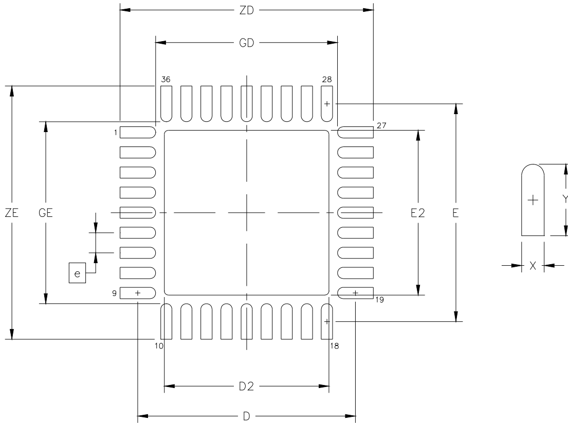
Figure 7. PCB Land Pattern Diagram
