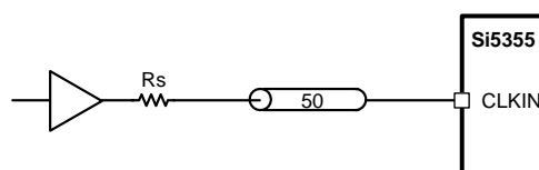
Figure 2. Interfacing CMOS Reference Clocks to the Si5355
