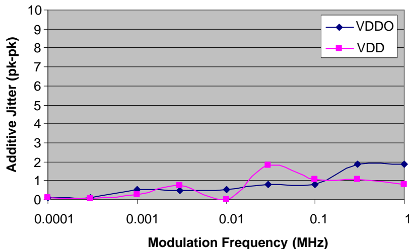
Figure 4. Peak-to-Peak Additive Jitter from 100 mV Sine Wave on Supply
