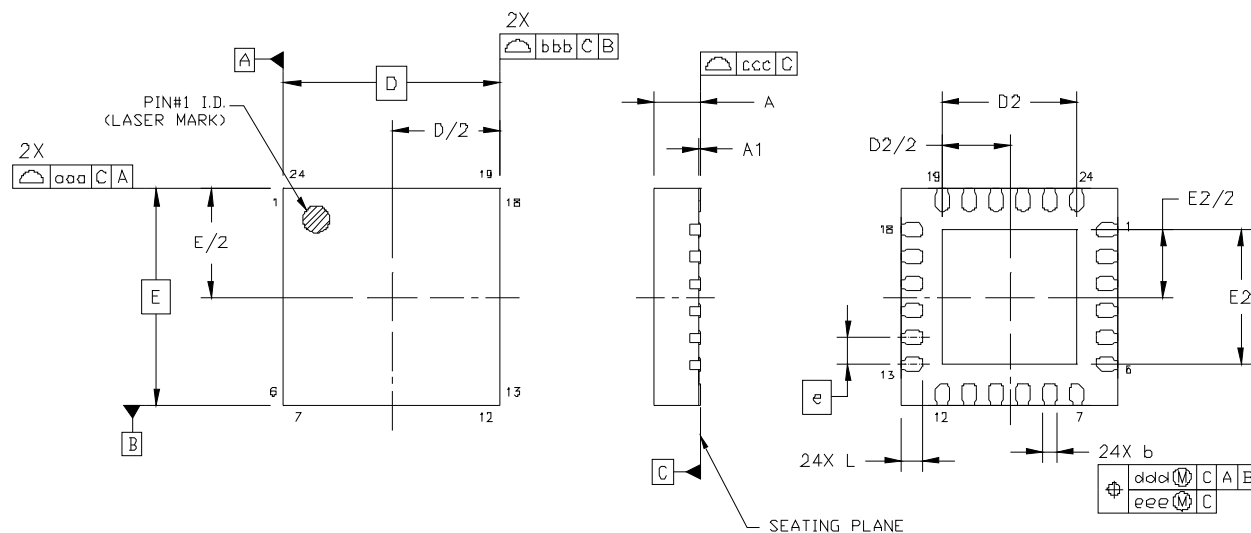
Figure 5. 24-Lead Quad Flat No-Lead (QFN)
