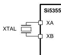
Figure 1. Connecting an XTAL to the Si5355
