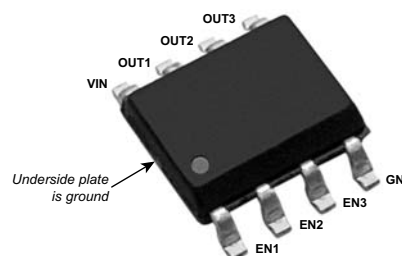
8-Lead Power SOIC (SG)
